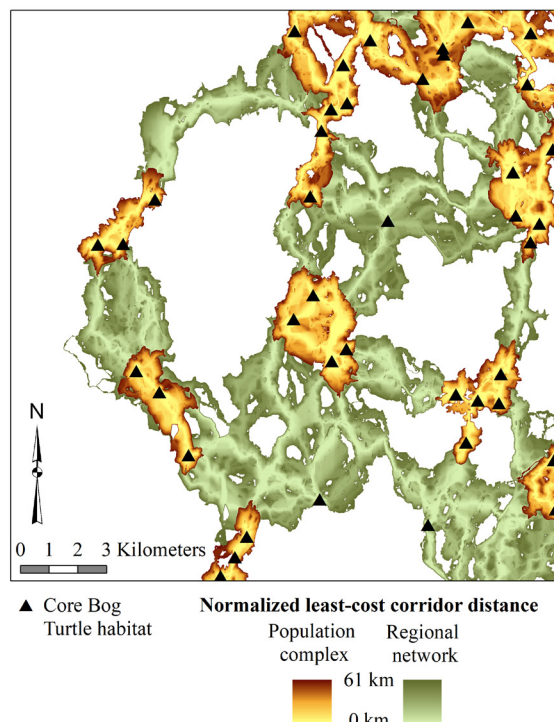
FIGURE 1. Normalized least-cost corridors among potential Bog Turtle ( Glyptemys muhlenbergii ) core habitats within maximum straight-line Euclidean distances of 2 km (population complex) and 10 km (regional network) in part of the New York study area (white). We instructed the model to connect each core to its three nearest neighbors and then to connect neighboring constellations. Corridor width was limited to 61 km cost-weighted distance. Exact locations protected due to the threat of poaching.
