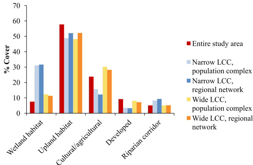
FIGURE 3. Percentage cover of select landscape features within two modeled least-cost corridors (population complex and regional network; see Fig. 1) connecting core Bog Turtle ( Glyptemys muhlenbergii ) habitats in the New York study area, and within the study area as a whole (590 km 2 ). Narrow corridors (maximum cost-weighted distance [CWD] width of 7.6 km) were generally 50–400 m and wide corridors (maximum CWD of 61 km) were generally 500–2,500 m in width.
