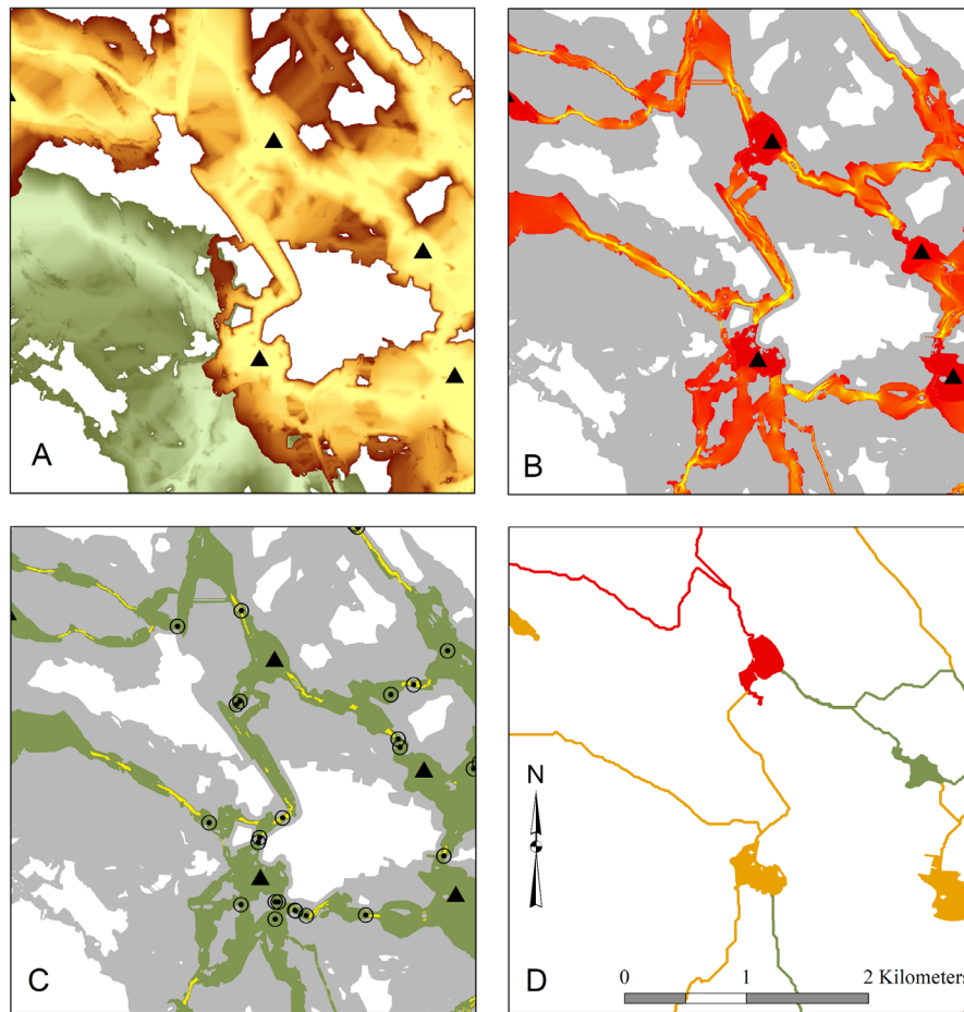
FIGURE 4. (A) Least-cost corridors among potential core Bog Turtle ( Glyptemys muhlenbergii ) habitats (black triangles) in part of New York study area for population complex model (lowest resistance routes in yellow, highest in brown) and regional network model (lowest resistance routes in light green, highest in dark green; see Fig. 1). (B) Current flow for both models constrained to a narrow version of the same least-cost corridors (maximum cost-weighted distance [CWD] width of 7.6 km), with highest current densities in yellow. Gray area corresponds to wide corridors (maximum CWD of 61 km) for both models. (C) Pinch points (yellow) defined as highest 10% of current values, and corridor outlines of wide (gray) and narrow (green) least-cost corridors. Intersections of corridors and roads marked with circled black points. (D) Core habitats and least-cost paths classified by centrality, the importance of each in keeping the whole network connected (lower centrality in green, higher in red), for the regional network model.
