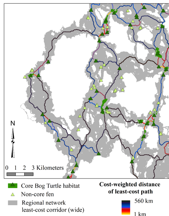
FIGURE 2. Cost-weighted distances of least-cost paths among potential Bog Turtle ( Glyptemys muhlenbergii ) core habitats within a maximum straight-line Euclidean distance of 10 km (regional network) in part of the New York study area. We instructed the model to connect each core to its three nearest neighbors and then to connect neighboring constellations. Corridor width was limited to 61 km cost-weighted distance. Exact locations protected due to the threat of poaching.
